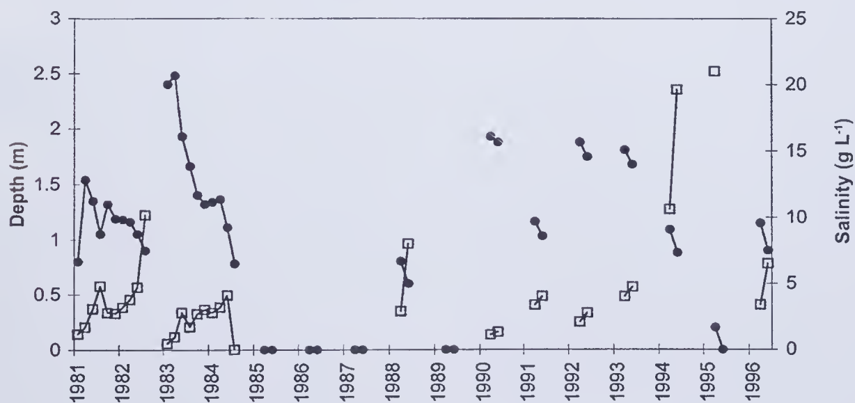
Figure 2. Depth (●) and salinity (□) at Toolibin Lake at 2-monthly intervals from July 1981 to May 1995 and each September and November thereafter (unpublished data, J A K Lane, Department of Conservation and Land Management), except in 1996 when December data are used instead of November (modified from Freund et al. 1997)
